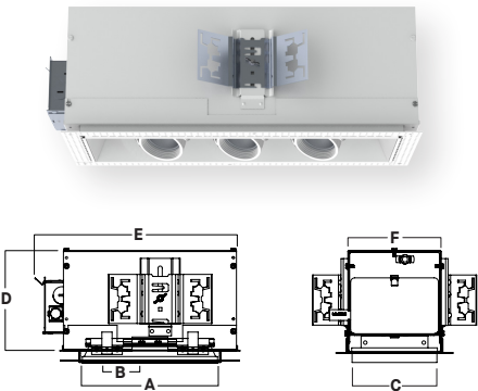
RC4_LVNF - REGRESSED RAZOR EDGE FLANGELESS
