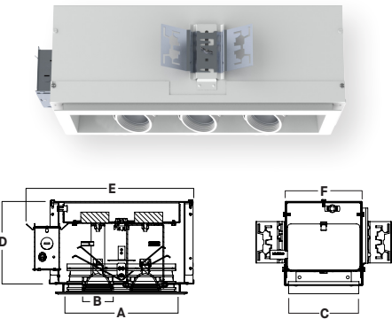
RC4_LVRT - REGRESSED BEVEL FLANGE
