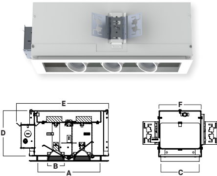
RC4_LVFT - FLUSH FLAT FLANGE
