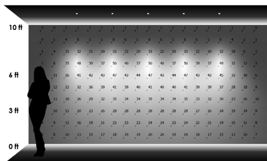
THREE LUMINAIRES 3'-0" away from wall 4'-0" on center
