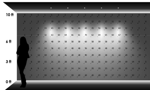
THREE LUMINAIRES 2'-6" away from wall 4'-0" on center
