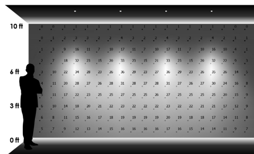
THREE LUMINAIRES 3'-6" away from wall 4'-0" on center
