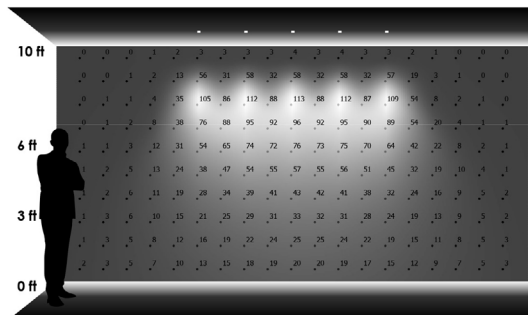
THREE LUMINAIRES 2'-0" away from wall 4'-0" on center
