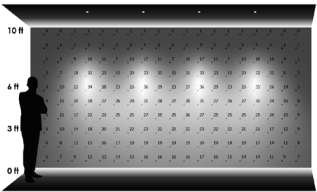
THREE LUMINAIRES 3'-6" away from wall 4'-0" on center
