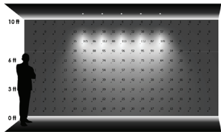
THREE LUMINAIRES 2'-0" away from wall 4'-0" on center
