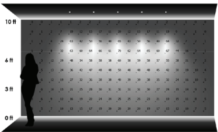
THREE LUMINAIRES 2'-6" away from wall 4'-0" on center
