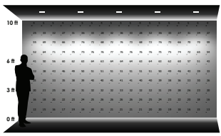
FIVE LUMINAIRES 3'-0" away from wall 4'-0" between luminaires
