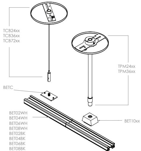
BET90 FLOATING CANOPY
