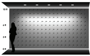
FIVE LUMINAIRES 3'-0" away from wall 3'-0" between luminaires
