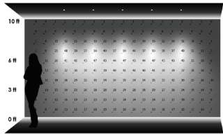
THREE LUMINAIRES 3'-0" away from wall 4'-0" on center
