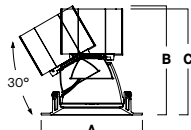
AA - 30° Adjustable Shallow Flange
