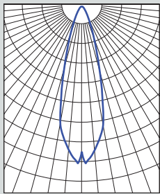
D4SQMH39w-Efficiency: 90.9% Spacing: 0.54
