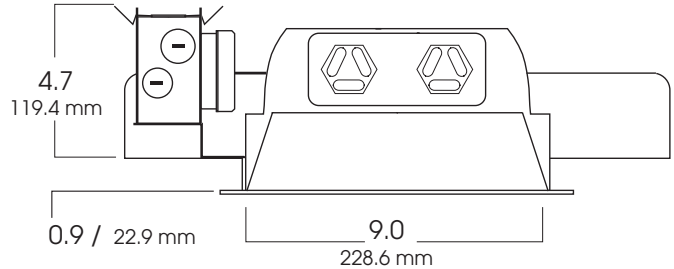
CROSS-SECTION
