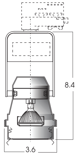
TEK100/HTEK100 adaptors for use with TEK/HTEK/XTS TRACK
