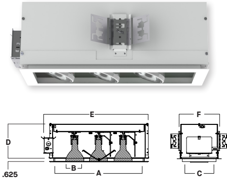
RC6_FTINC PAR30 - FLUSH FLAT FLANGE
