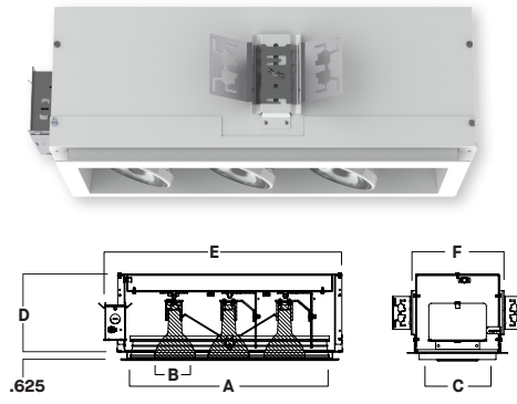
RC6_RTINC PAR30 - REGRESSED BEVELED FLANGE
