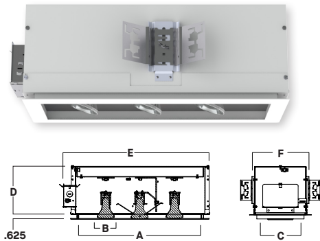
RC6_FTINC PAR20 - FLUSH FLAT FLANGE
