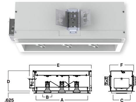
RC6_RTINC PAR20 - REGRESSED BEVELED FLANGE
