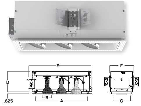
RC6_NFINC PAR30 - REGRESSED RAZOR EDGE FLANGELESS
