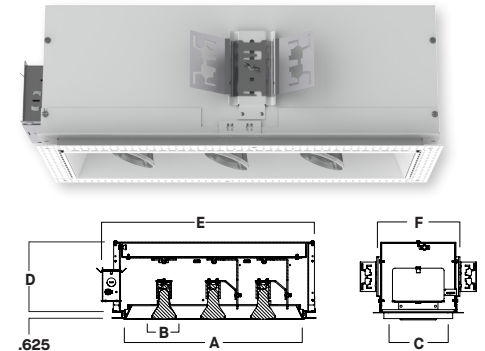
RC6_NFINC PAR20 - REGRESSED RAZOR EDGE FLANGELESS
