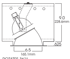
SGA7MH -7" T4 /T6 METAL HALIDE ADJUSTABLE - UV PROTECTED
