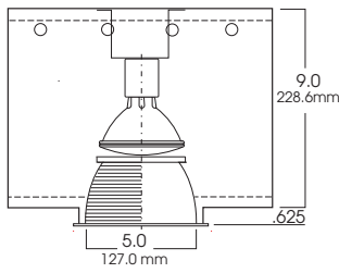
SGD5MH 5" APERTURE PAR30 METAL HALIDE DOWNLIGHT
