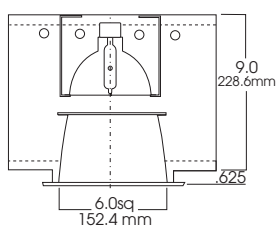
SGD6SQMH -6" SQ. T4/T6 METAL HALIDE DOWNLIGHT - UV PROTECTED
