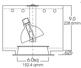
SGA6SQMH -6" SQ. T4/T6 METAL HALIDE ADJUSTABLE - UV PROTECTED
