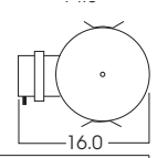
HOUSING Ø11.5 X 16.0 OVERALL
