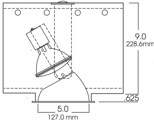
SGA5MH 5" APERTURE PAR30 METAL HALIDE ADJUSTABLE
