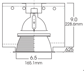
SGD7MH -7" T4 /T6 METAL HALIDE DOWNLIGHT - UV PROTECTED
